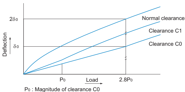
Fig.10 Rigidity Data
