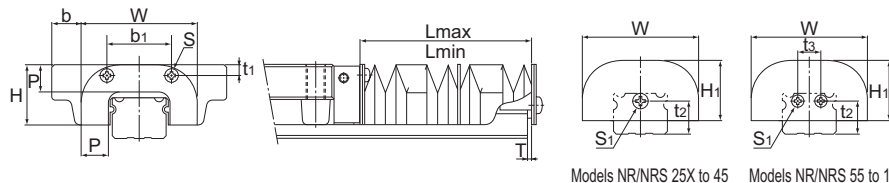
Models NR/NRS 25X to 45 Models NR/NRS 55 to 100
